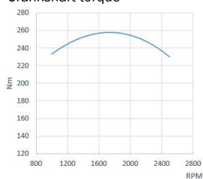
Crankshaft torque
